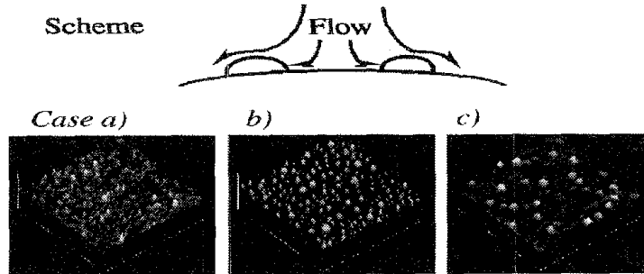
FIG. 1. The scheme of flow over a rough surface is shown schematically in the top portion of this figure. In the bottom panels, AFM images are shown of the following cases: (a) self-assembled OTS layers; (b) PS/PVP-OTE layers (surface coverage \sim 80\% ); (c) PS/PVP-OTE layers (surface coverage \sim 20\% ). Each AFM image concerns an area 3 \mu\text{m} \times 3 \mu\text{m} .
